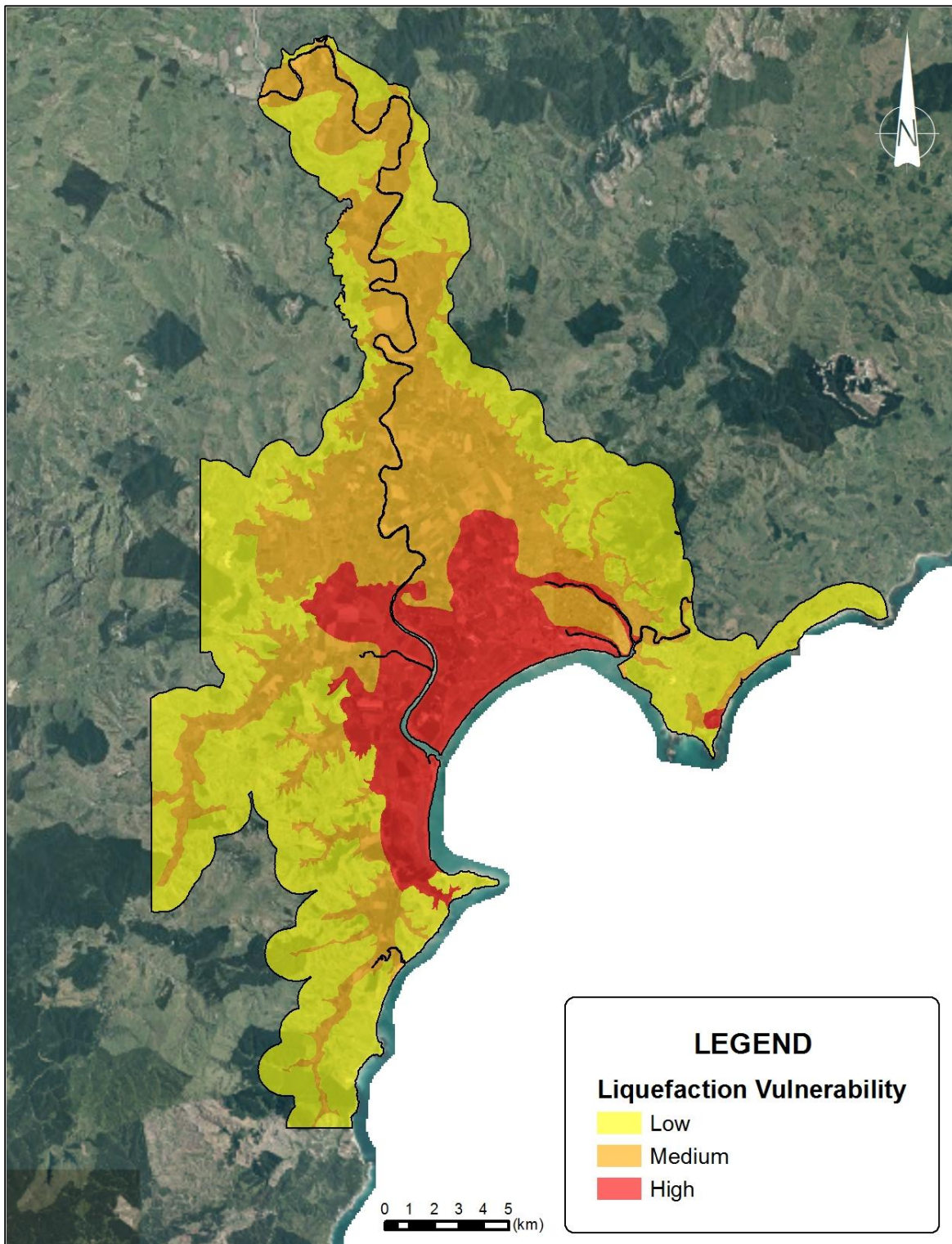
Figure 5-2: Map showing liquefaction vulnerability for the study area
